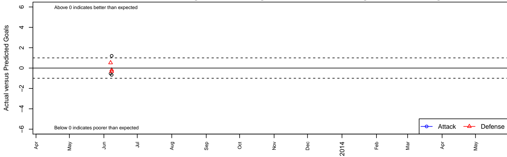
3 Rivers ThielemannB02 Dots are actual minus expected GF (blue circles) and GA (red triangles). Blue line is smoothed change in attack strength. Red is smoothed change in defense strength.
